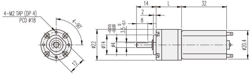
GEARHEAD LENGTH
